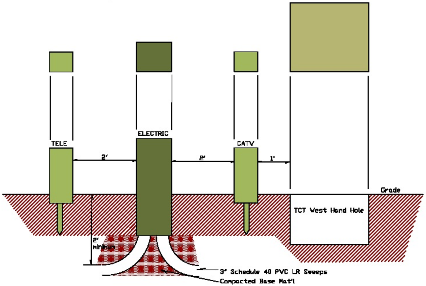
Secondary Pedestal & Telecommunications Template
